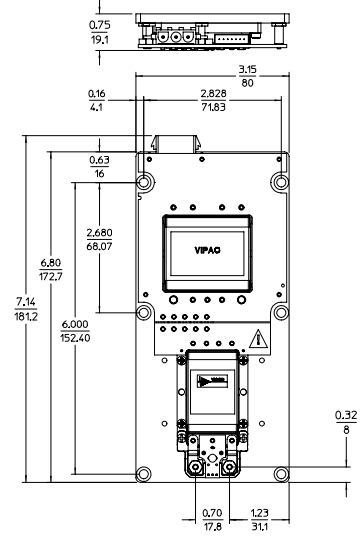
Configuration MVC-G / MVX-G LugMates
