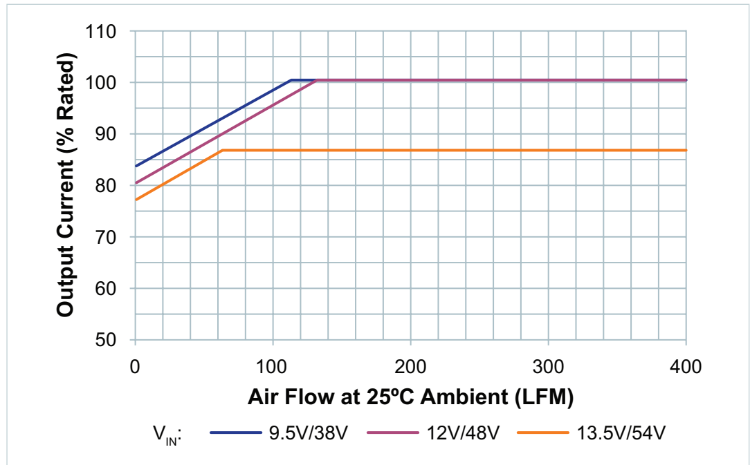
Figure 5 Output current versus required airflow for NBM2317S54D1464TOR mounted on evaluation board demo assembly at 25°C ambient
